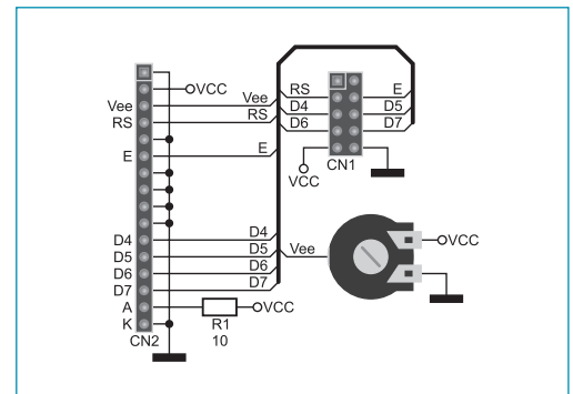
Figure 4: LCD Adapter additional board connection schematic
