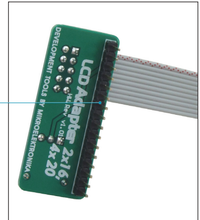
Figure 2: LCD Adapter board's back view
