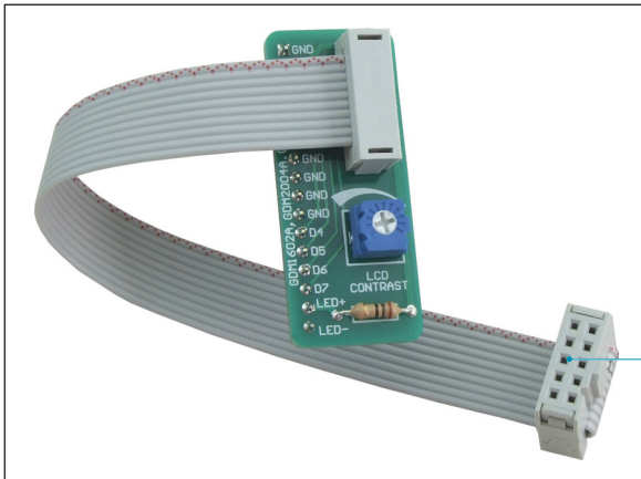
Figure 1: LCD Adapter additional board
