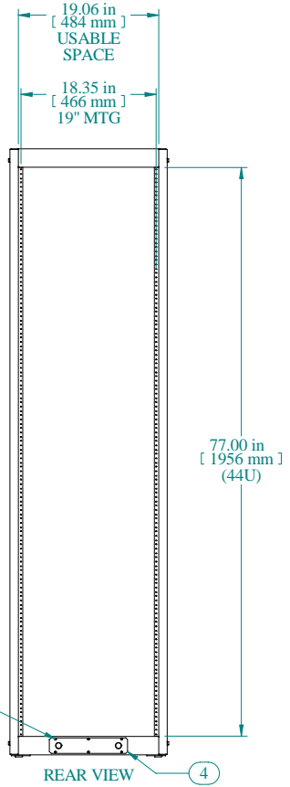
REAR VIEW
