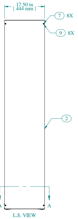
L.S. VIEW
