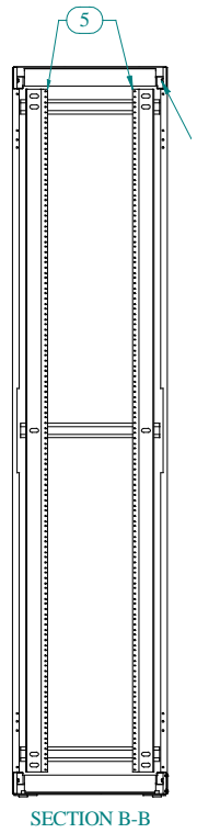
SECTION B-B
