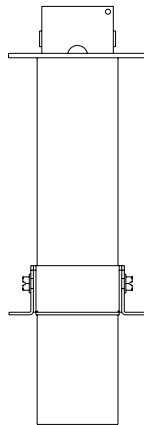
BOTTOM VIEW
